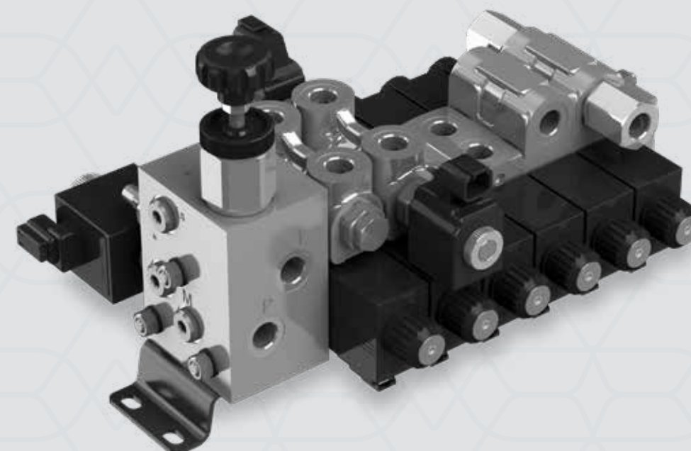
SDE030 - SDE060 Bankable solenoid valves
