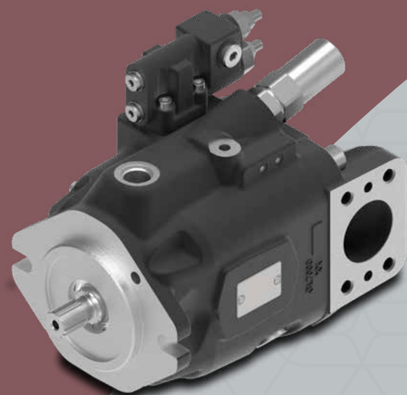
PWLS Variable displacement piston pump
